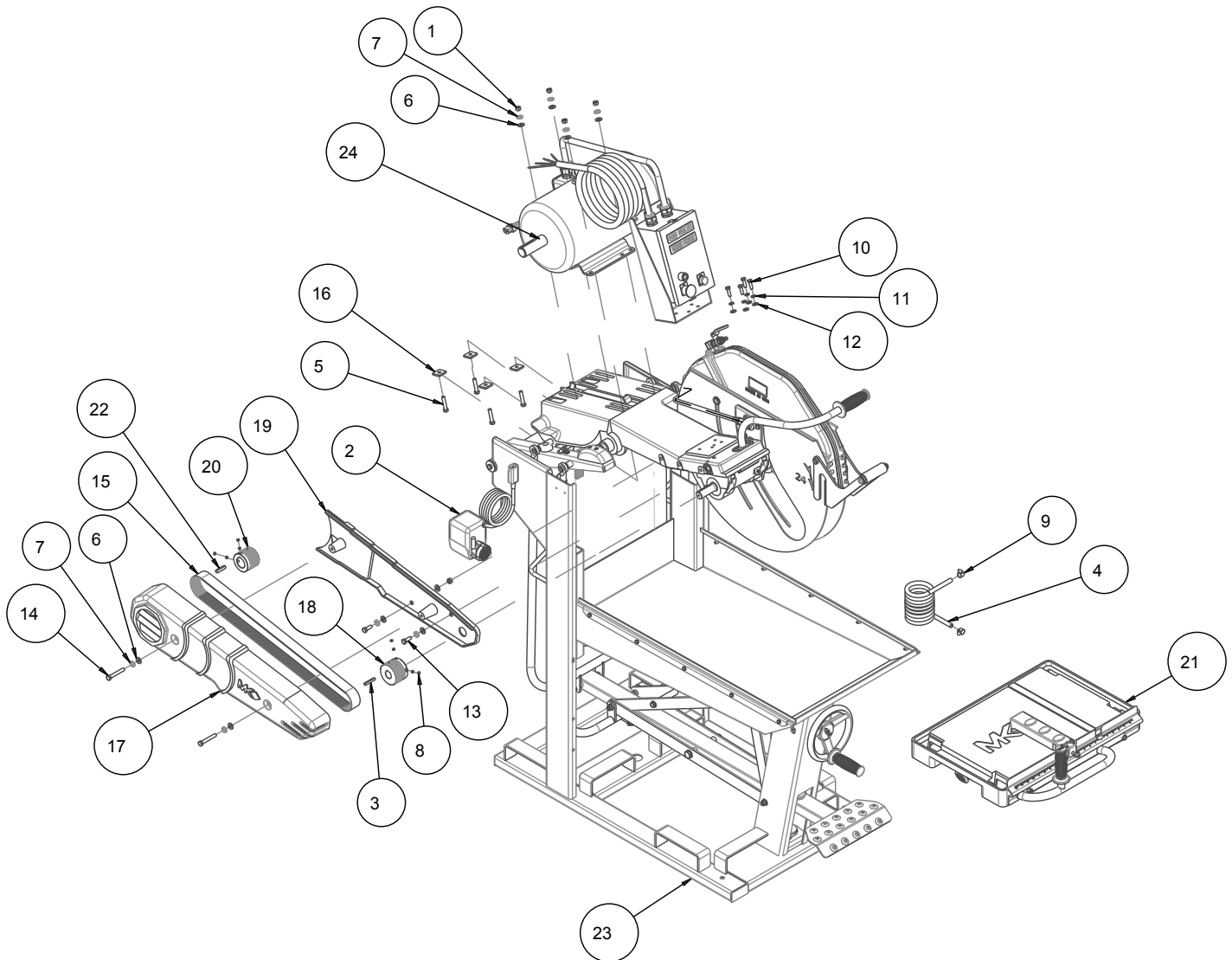
FIGURE 3 - MK-5010T SUPERMATIC BLOCK SAW 60 HZ/460V P/N 166931
