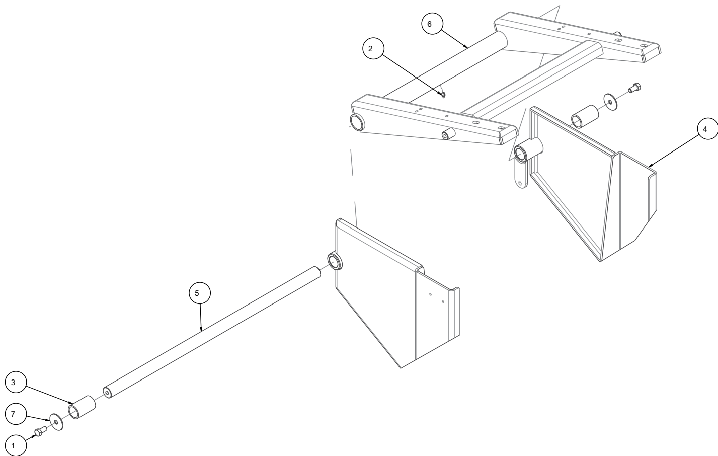
FIGURE 6 - MK-5000 ASSY, BLOCK SAW ELEVATOR ARM P/N 154629
