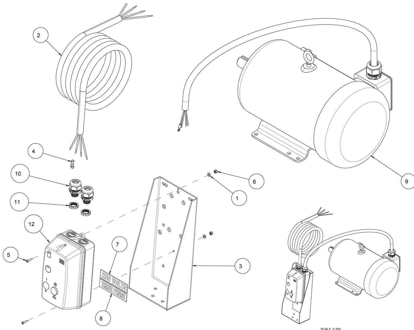
FIGURE 18 - MK-5000 ASSY, MOTOR, 10HP 230V 3 PH 1725RPM, EM3714T P/N 172772
