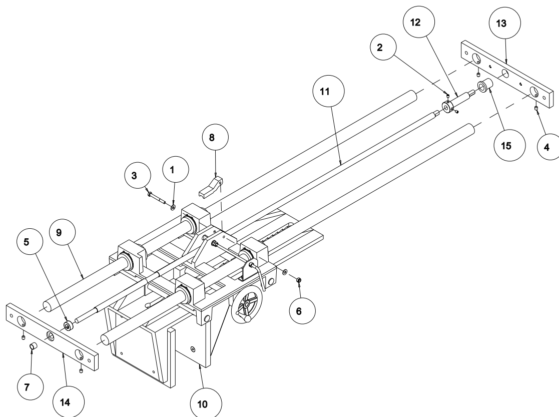
FIGURE 6 - HP30 ASSY. VISE P/N 173062
