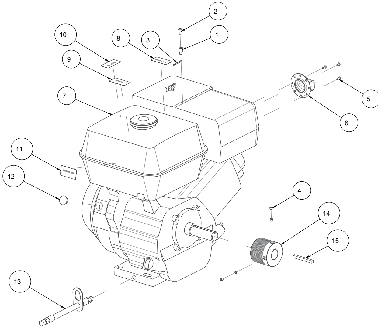
FIGURE 14 - MK-SG ASSY, ENGINE, HONDA, 9HP PART # 155396-MK
