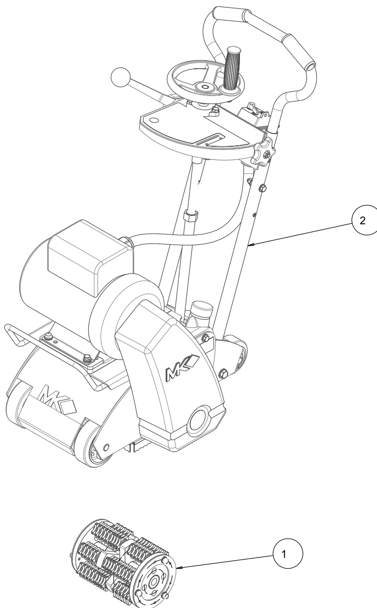
FIGURE 8 - MK SCARIFIER MK-SG-5H ELEC. W/6 POINT CARBIDE STAR PART #165277
