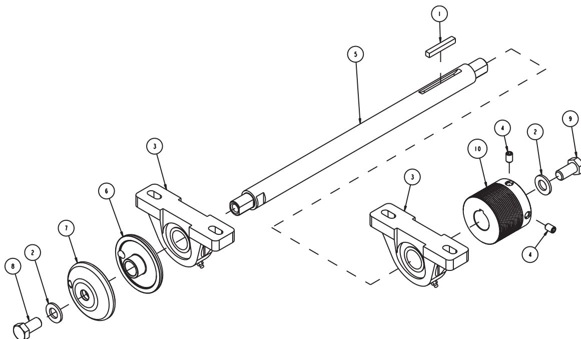
FIGURE 8 - ASSY, BLADE SHAFT - PART # 165977
