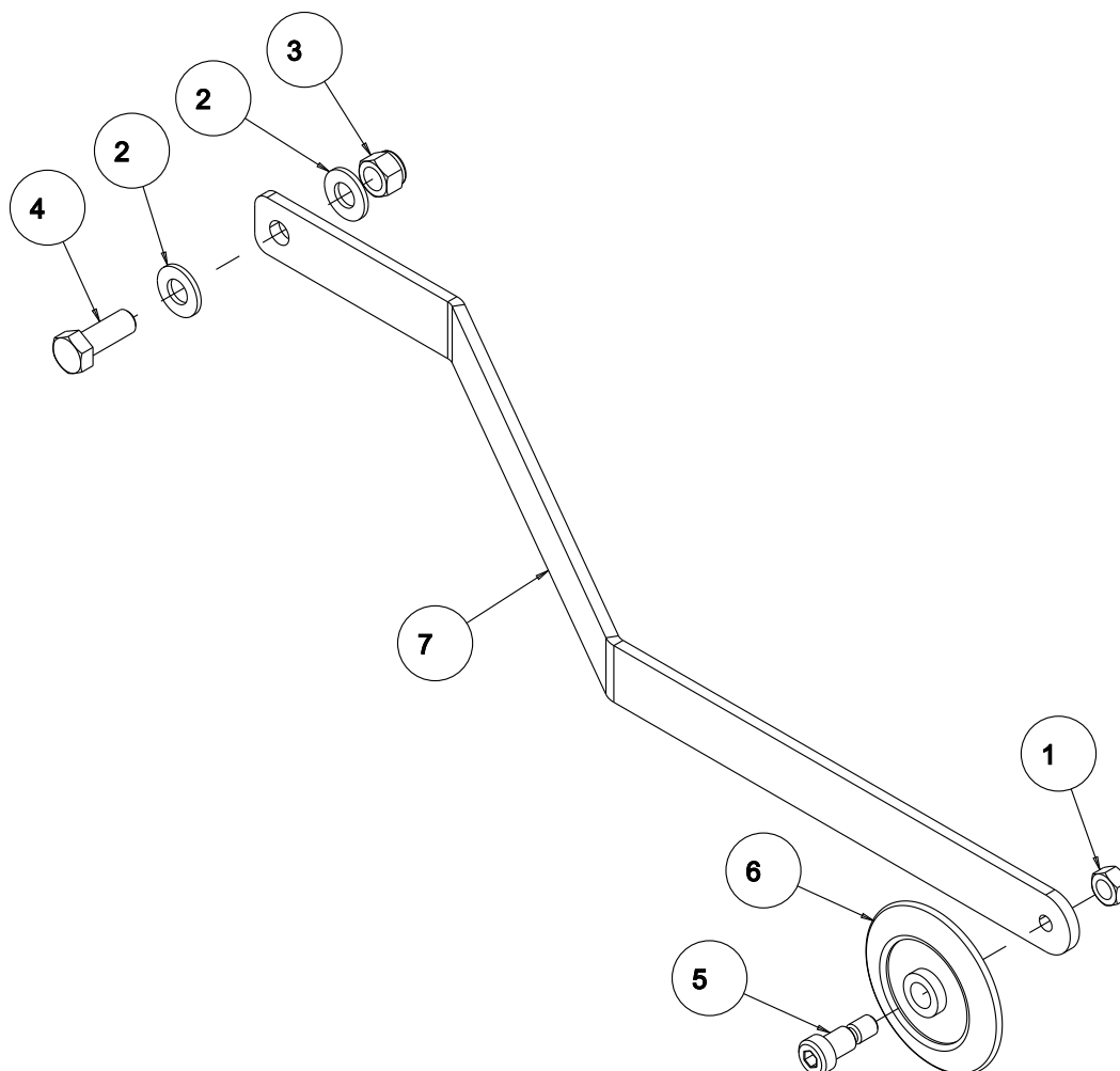
FIGURE 10 - PARTS LIST: ASSY, POINTER ARM - P/N 155568
