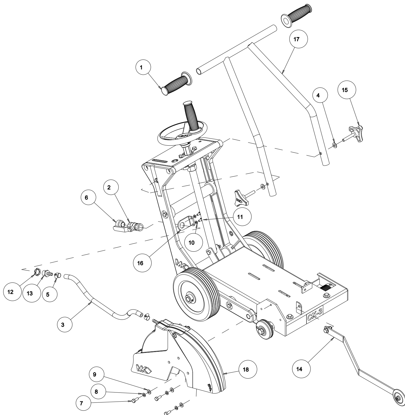
FIGURE 6 - PARTS LIST: MK-CX3 LESS ENGINE - P/N 165974X
