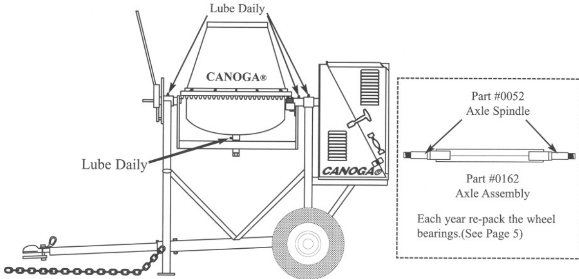
CANOGA® Equipment Model 100
