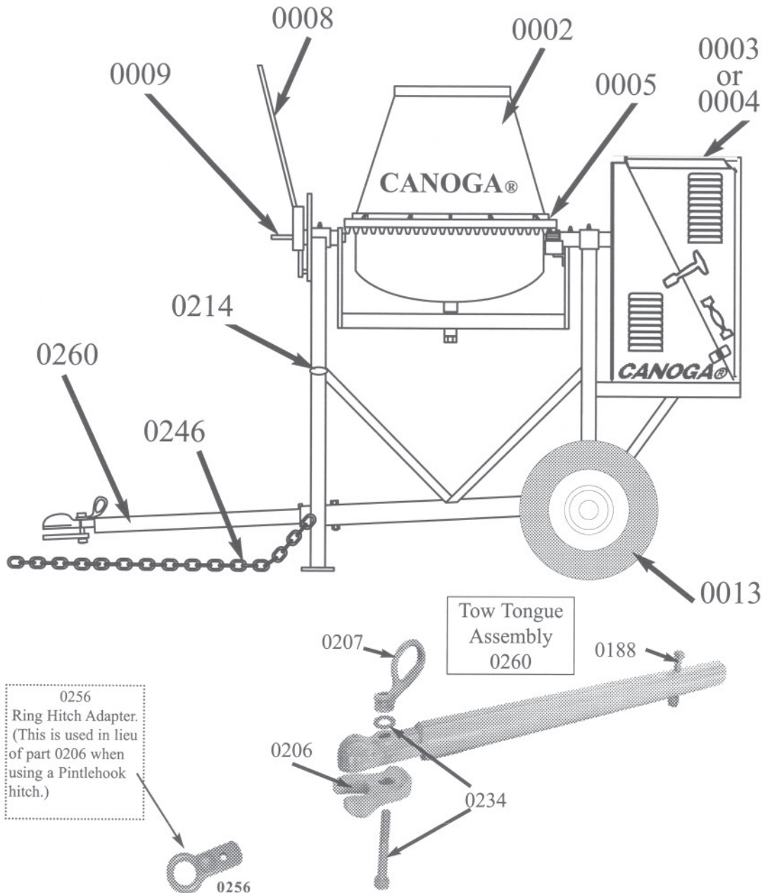
CANOGA® Equipment Model 100
