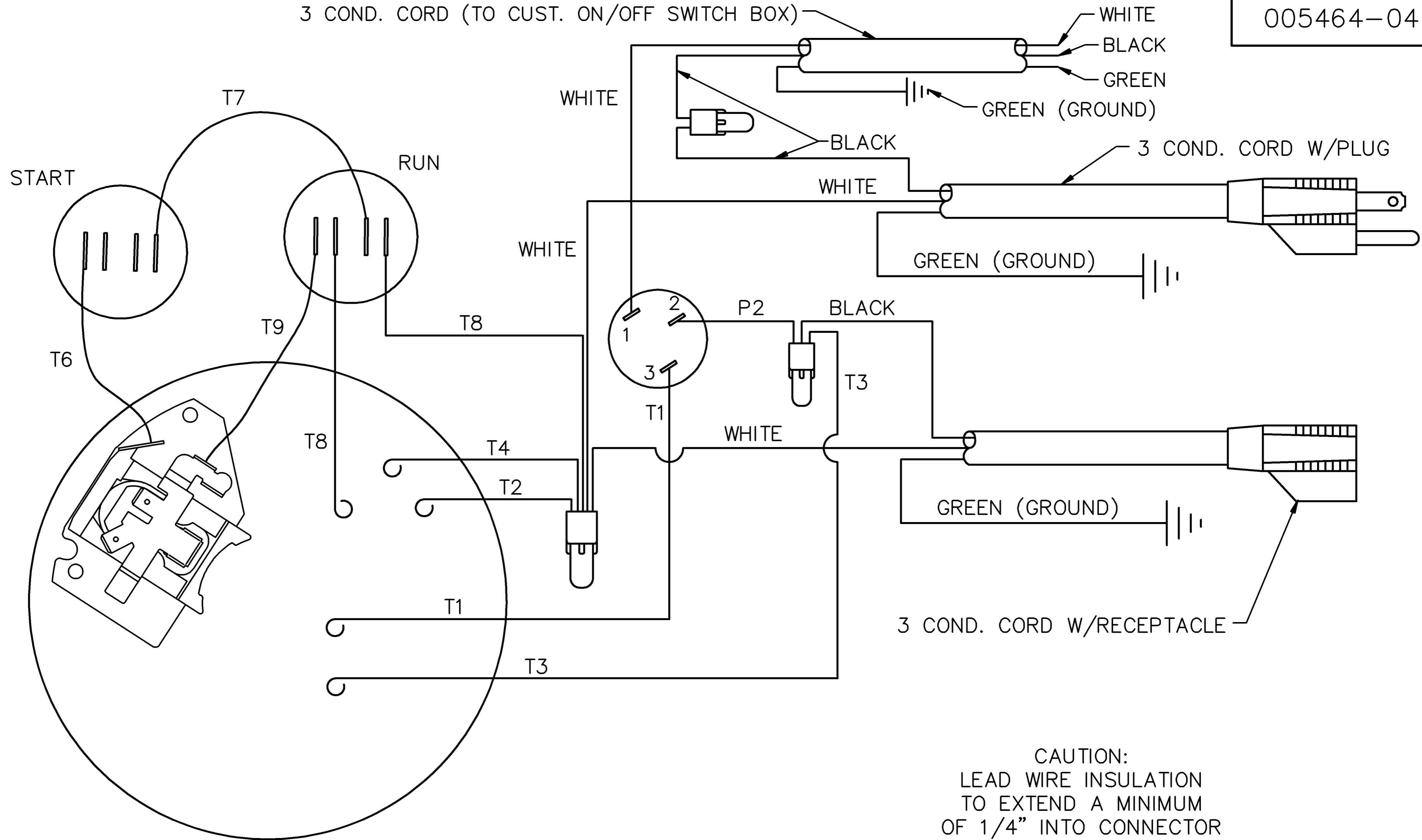
VIEW FROM OUTSIDE OF MOTOR AT SWITCH END.
