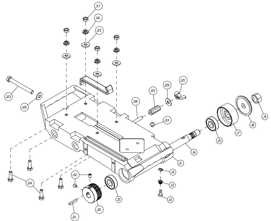
Sub-Assembly "J"
