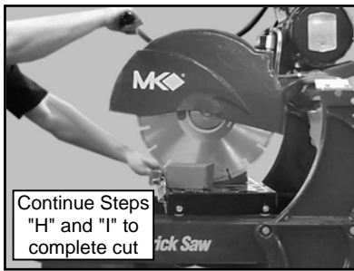
(J) Repeat steps H and I until cutting is complete
