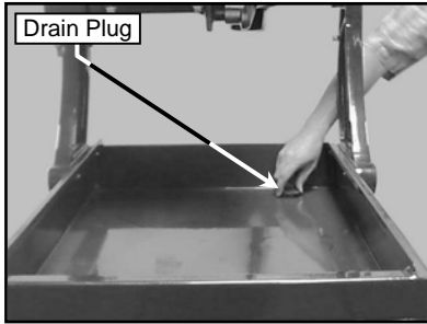
(H) Remove Drain Plug and dispose of water (conform to Federal, State and local laws for disposal)
