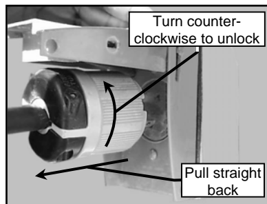
(E) Unplug the MK-2000 PRO Polarized plug from the power source by turning counter- clockwise and then pulling straight back
