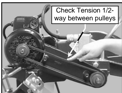
(G) Check the V-belts for proper tension, if the tension is correct, go to step R (Proper tension 1/8-inch deflection)
