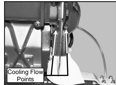
(C) Run the MK-2000 PRO until clear water is seen at the Blade cooling ports (Approx. 1 minute)
