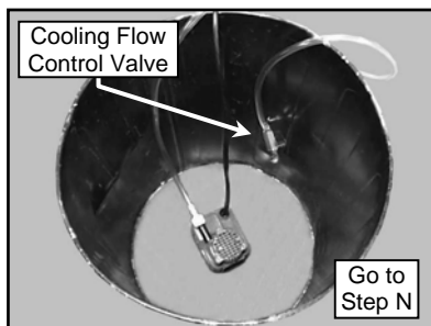
(J) Attach the Flow Control Valve to the Intake Fitting and check flow (See Step C)
