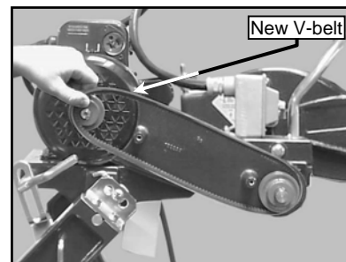
(L) Install the new V-belts (MK Part Number – 151723)
