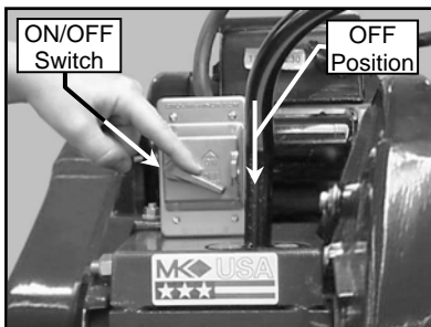
(K) Turn the Saw off when cutting is complete
