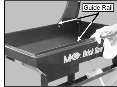
(J) Clean the Movable Cutting Table Guide Rails
