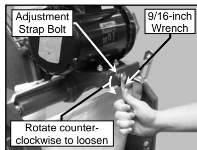
(I) Loosen the Motor Adjustment Strap using a 9/16-inch wrench
