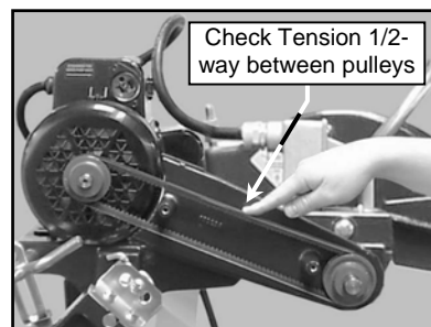
(O) Check the V-belts for proper tension, if the tension is correct, go to step R (Proper tension 1/8-inch deflection)
